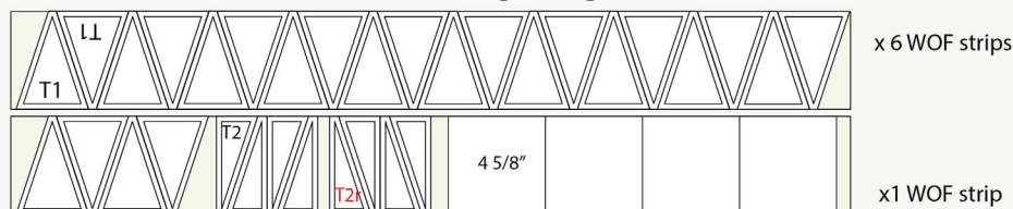
Fabric S Cutting Diagram
